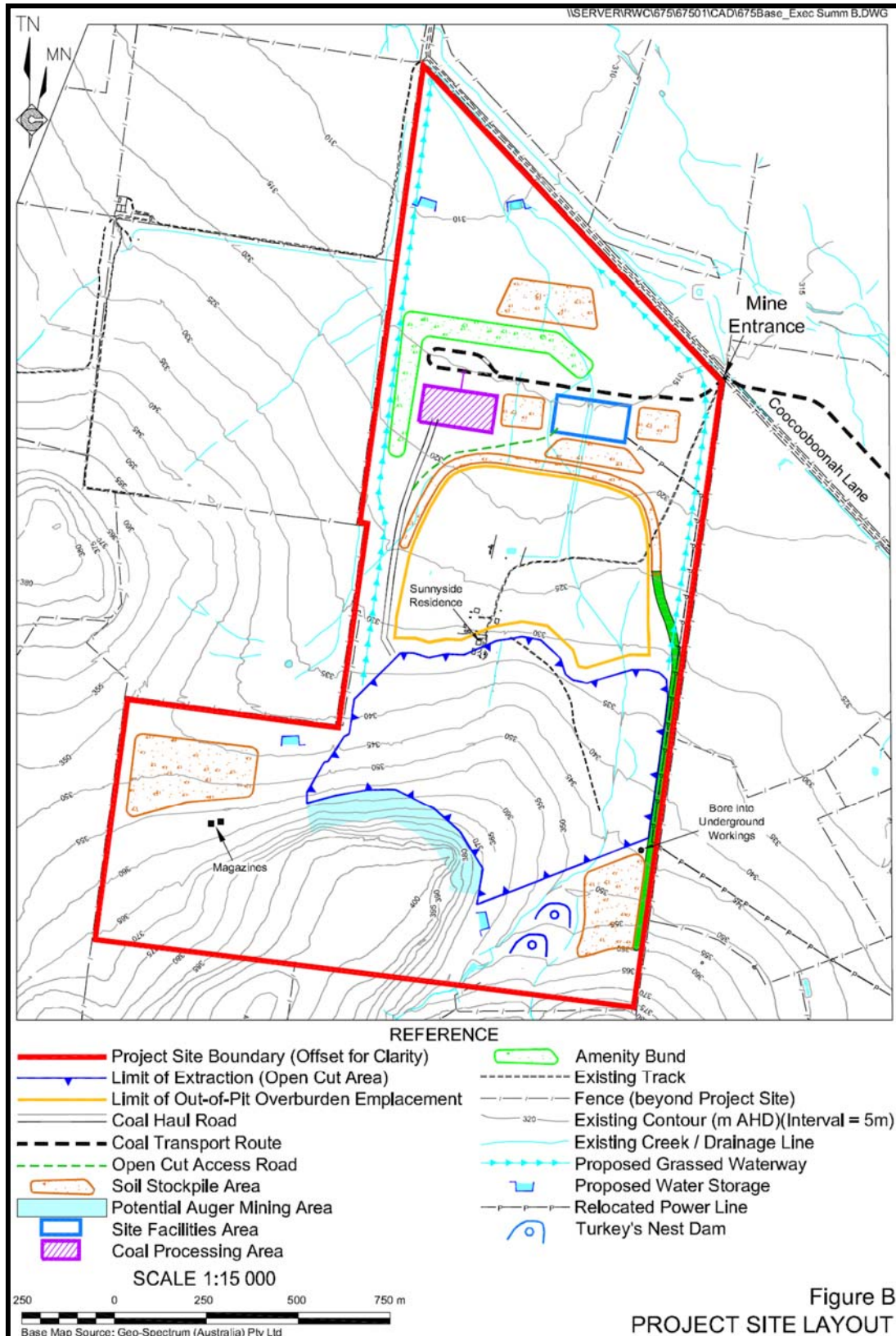
Figure 1: Project Layout
